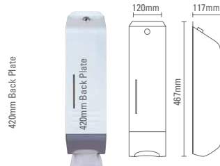
METAL DISPENSER - 4404 White enamel, lockable, tough for vandal-prone areas
